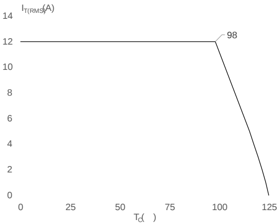
FIG.4: On-state character
