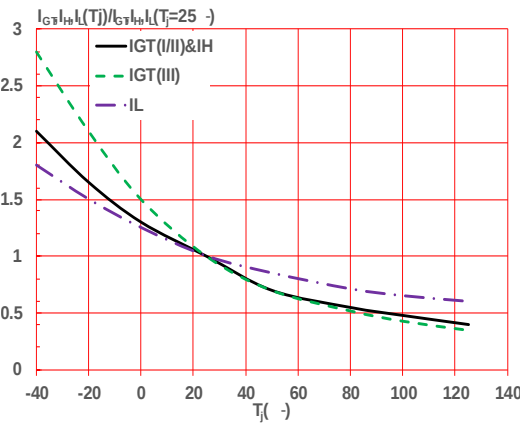
FIG.7: Relative holding current and latching current v junction temperature
