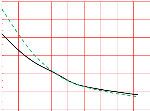
FIG.7: Relative variations of gate tri current, holding current and latchiurrent versus junct.77( )ion temperature
