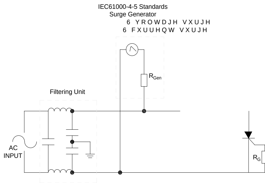
FIG.7 ÖTest circuit for inductive and resistive loads to IEC-61000-4-5 standards.
