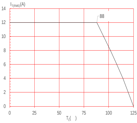
FIG.4: On-state characteristics
